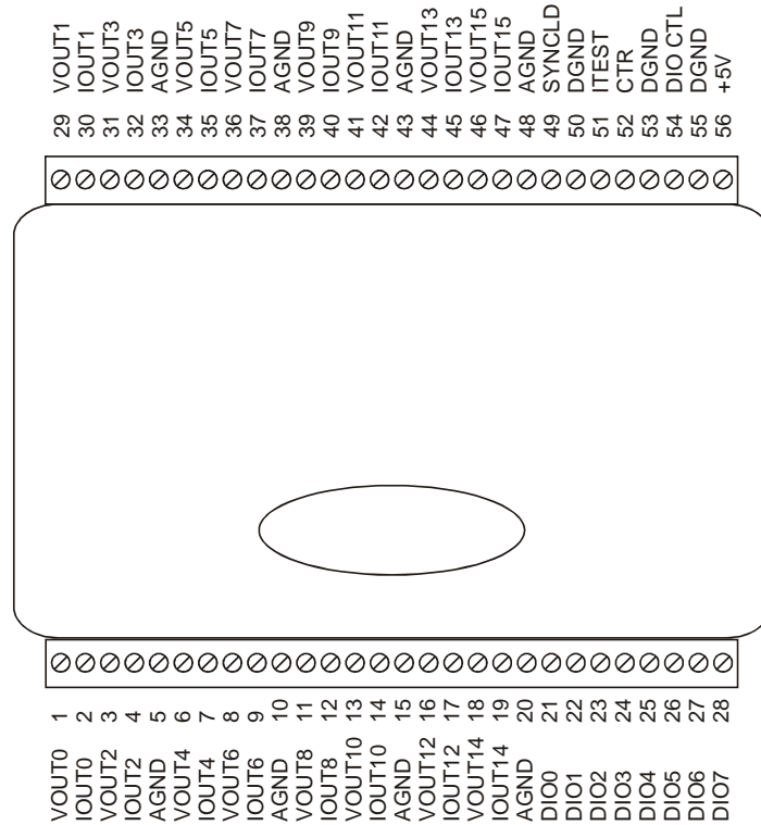
Figure 5. USB-3106 signal pin out
